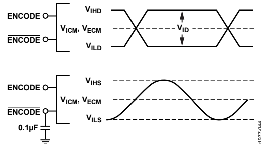
Figure 44. Differential and Single-Ended Input Levels
