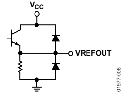
Figure 39. Voltage Reference Output Circuit
