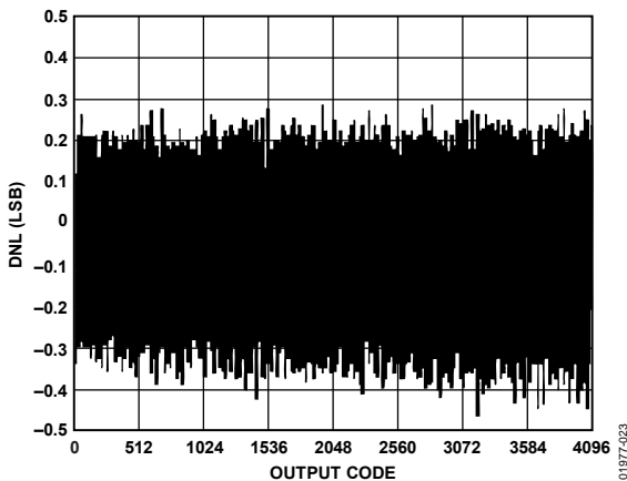
Figure 18. Differential Nonlinearity vs. Output Code
