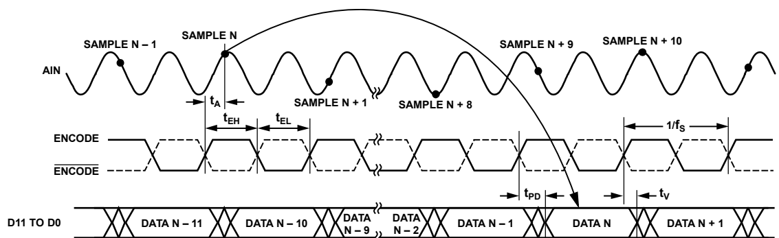
Figure 2. Timing Diagram
