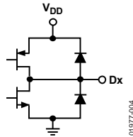
Figure 38. Digital Output Circuit
