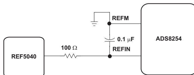
Figure 73. ADS8254 Using External Reference
