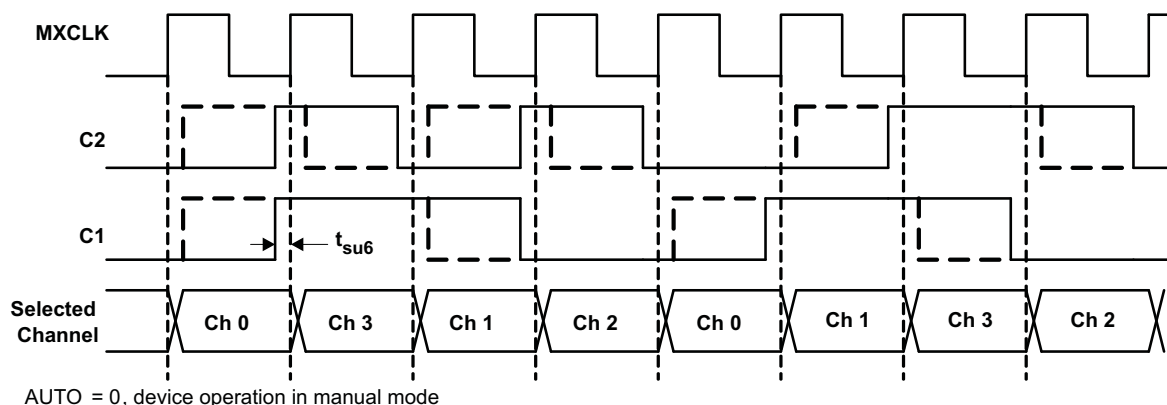
Figure 8. Multiplexer Manual Mode Timing Diagram
