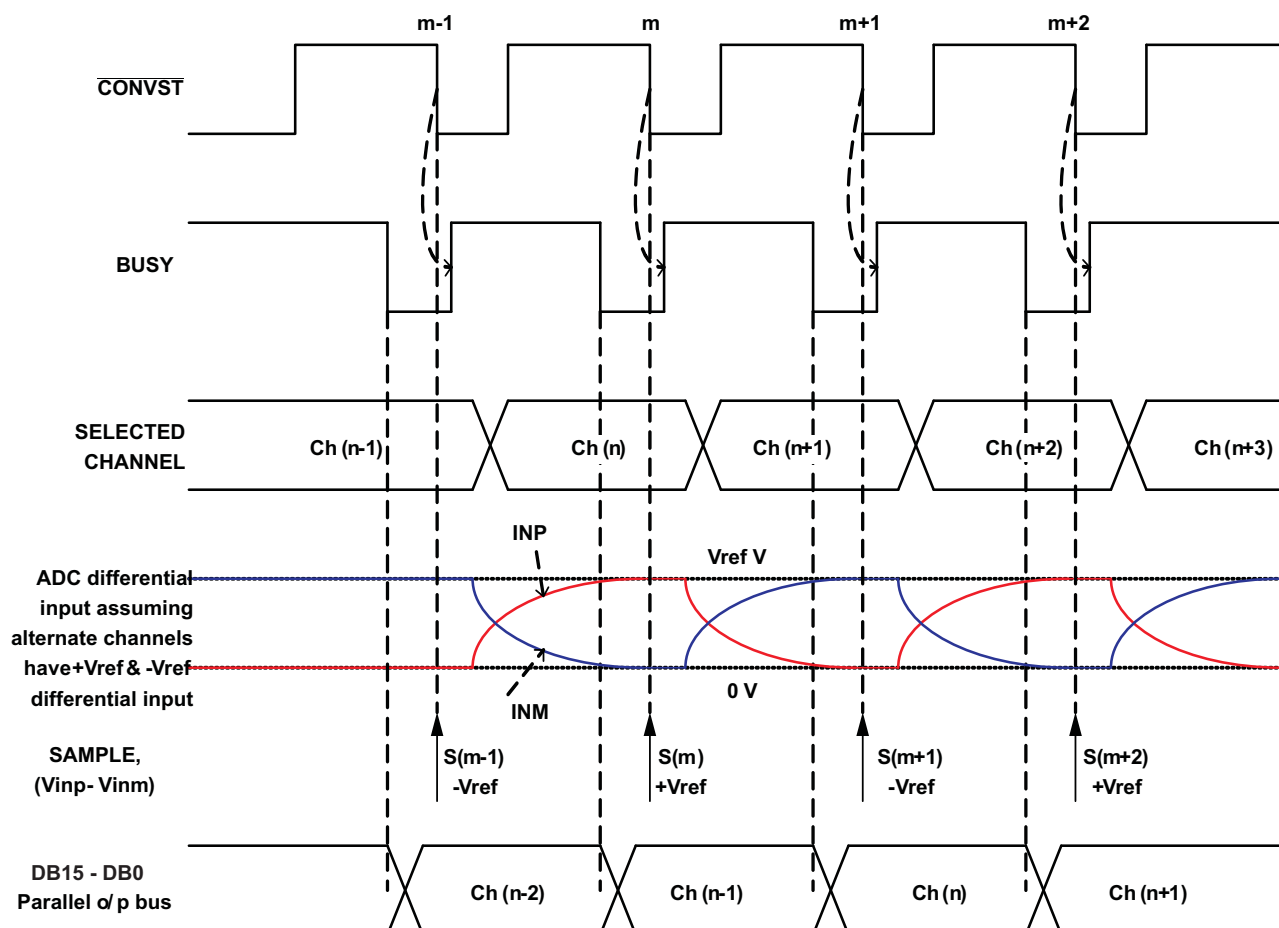
Figure 1. Device Operation
