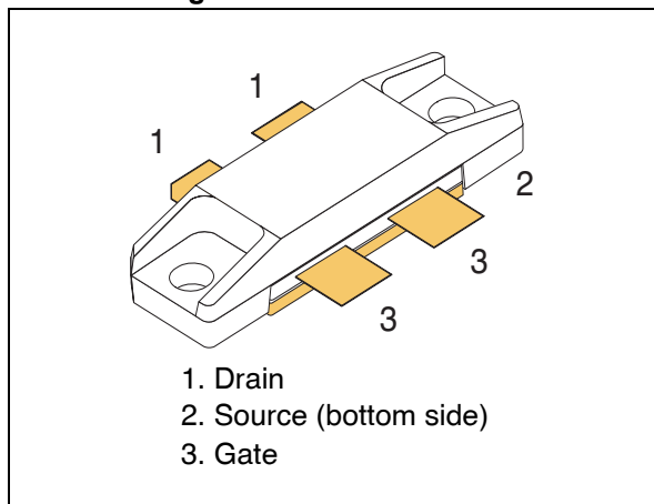
Figure 1. Pin connection
