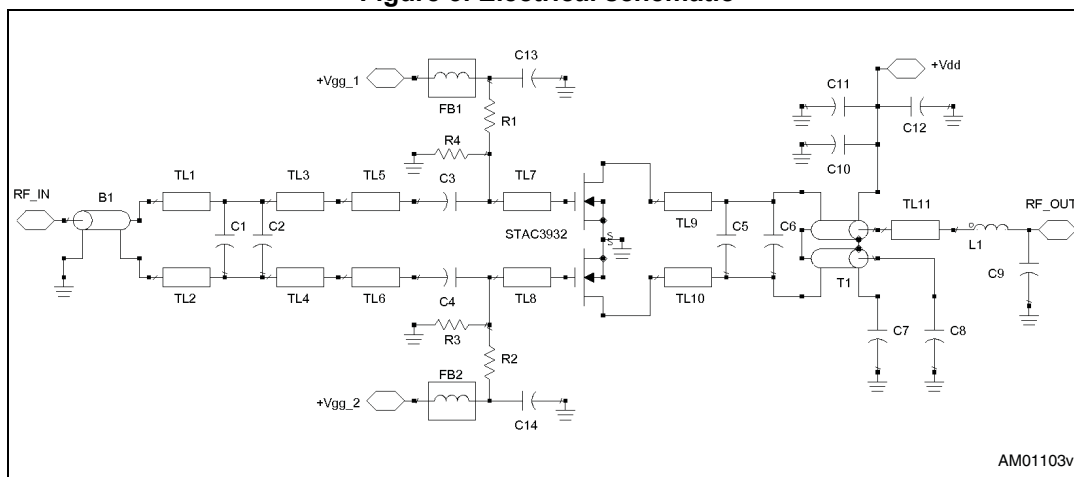
Figure 3. Electrical schematic
