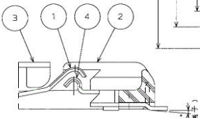
SECT. B-B (SCALE 5:1)
