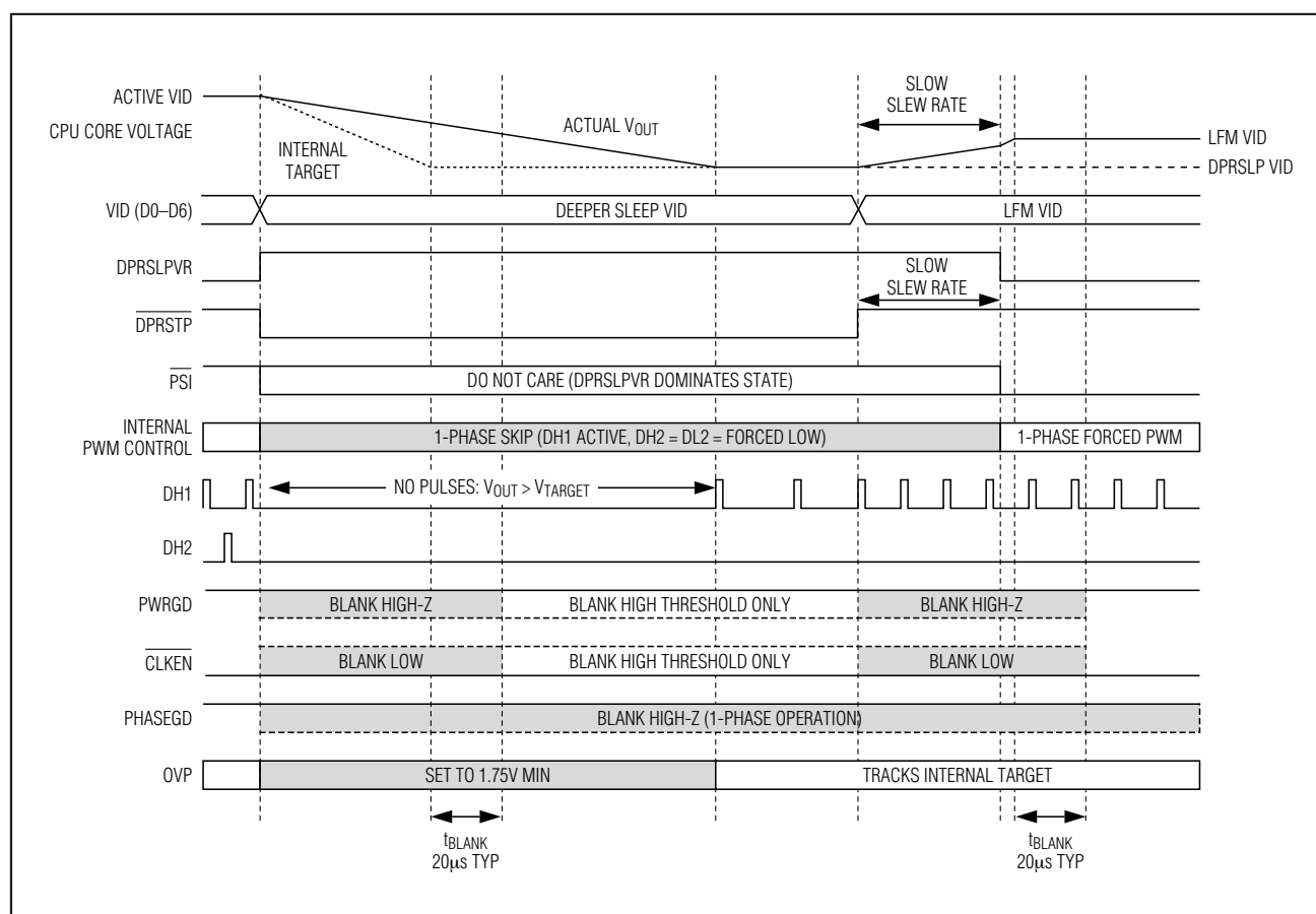
Figure 6. Slow C4 Transition
