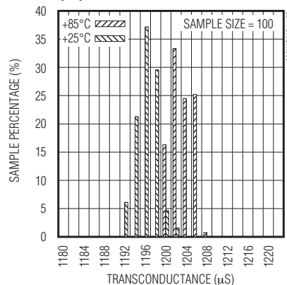
Gm(FB) TRANSCONDUCTANCE DISTRIBUTION
