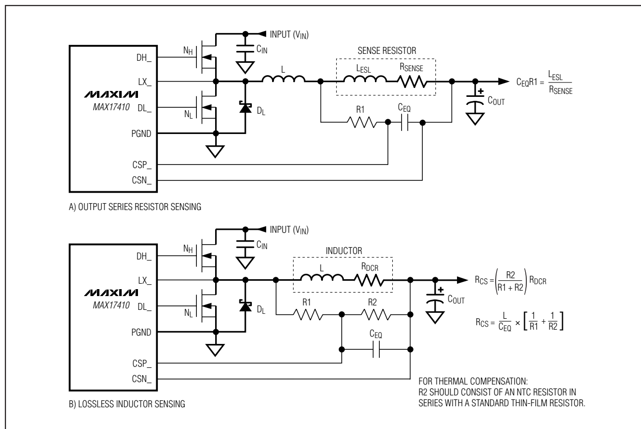
Figure 3. Current-Sense Methods
