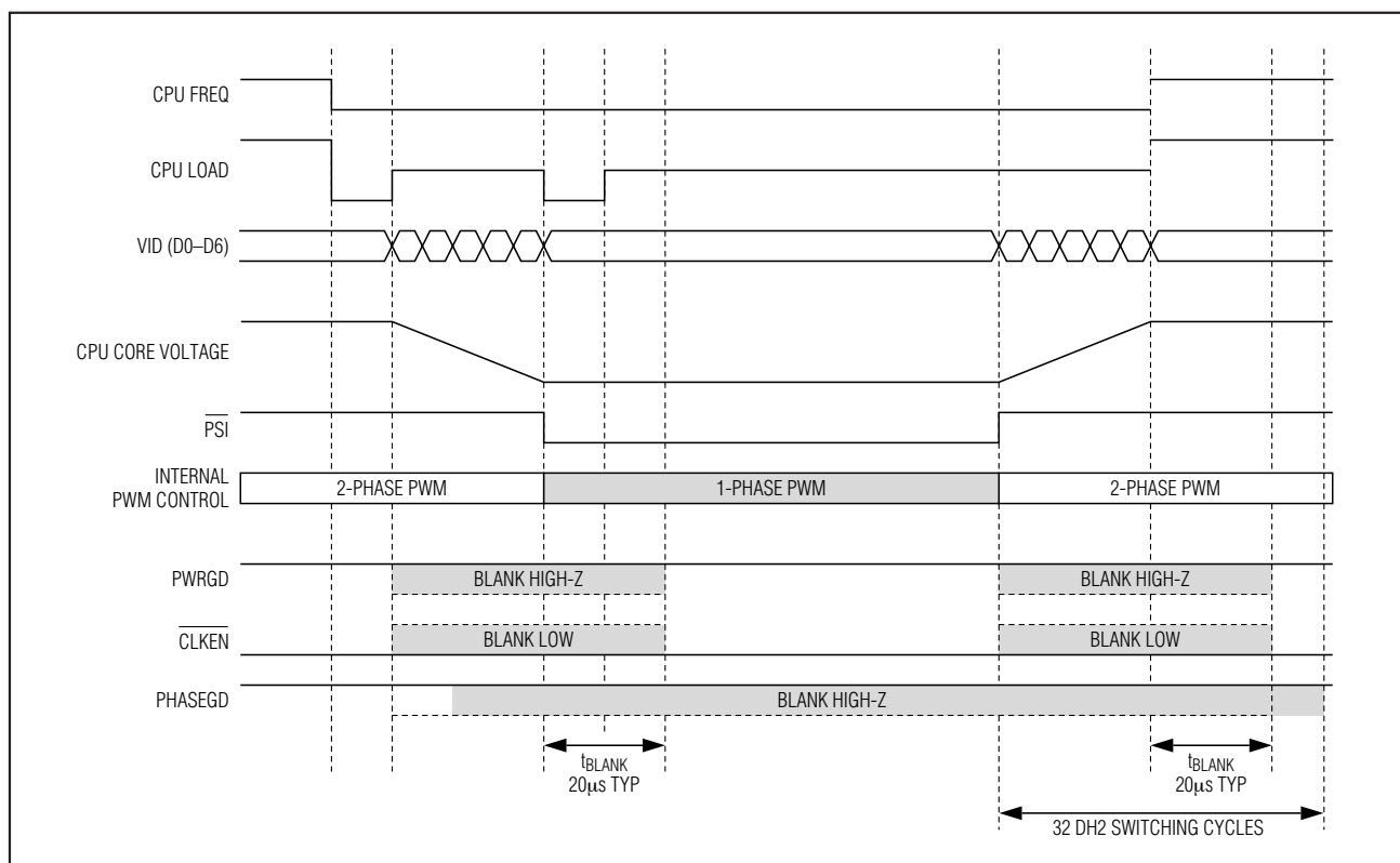
Figure 7. \overline{\text{PSI}} Transition
