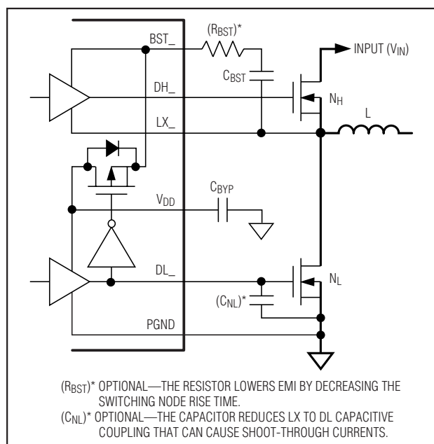
Figure 10. Gate-Drive Circuit
