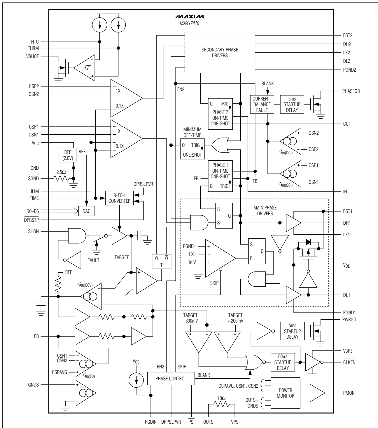
Figure 2. Functional Diagram
