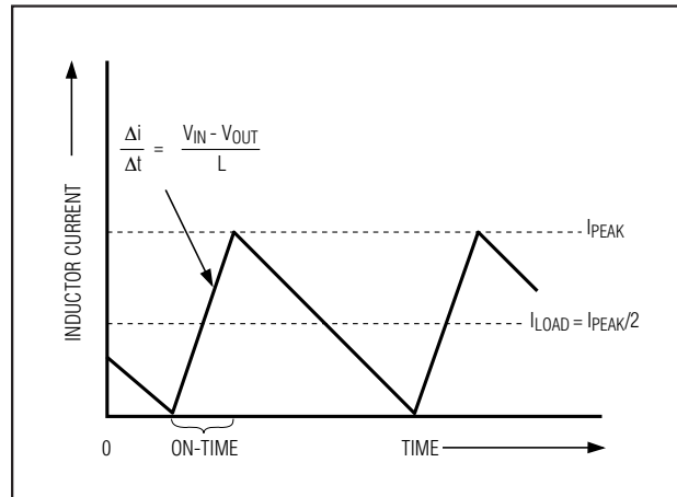
Figure 8. Pulse-Skipping/Discontinuous Crossover Point
