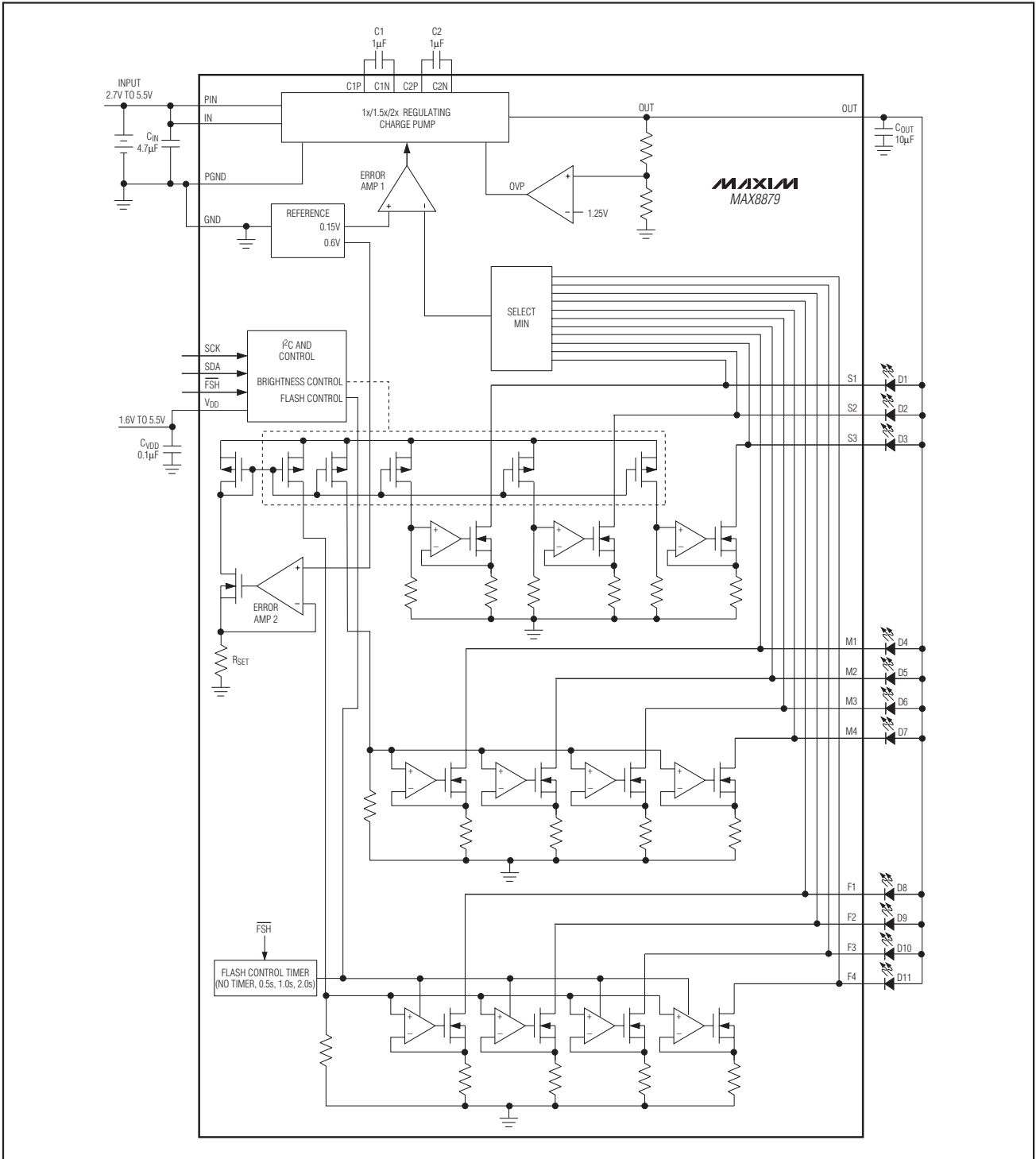
Figure 1. Functional Diagram
