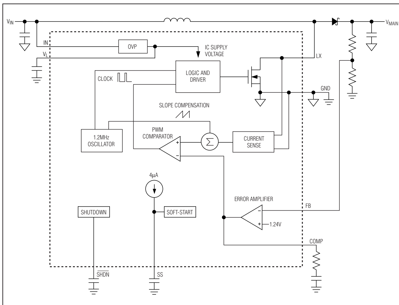
Figure 2. Functional Diagram
