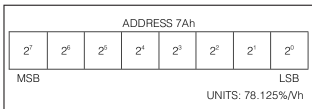
Figure 11. Initial Capacity Scaling Factor Register Format
