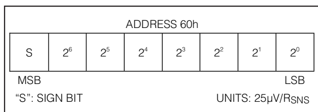
Figure 9. Current Offset Bias Register Format
