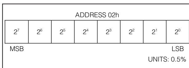
Figure 10. Relative Capacity Register Format
