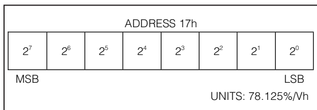
Figure 12. Learned Capacity Scaling Factor Register Format
