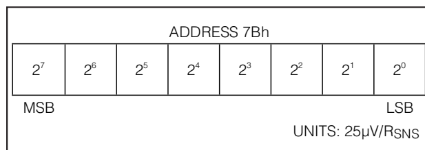
Figure 13. OCV Threshold Register Format
