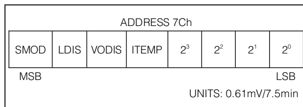
Figure 14. OCV dV/dt Threshold Register Format
