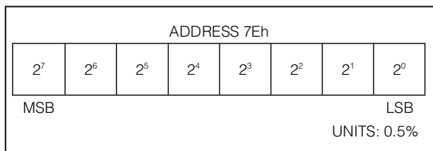
Figure 20. Learn Delta Percent Threshold
