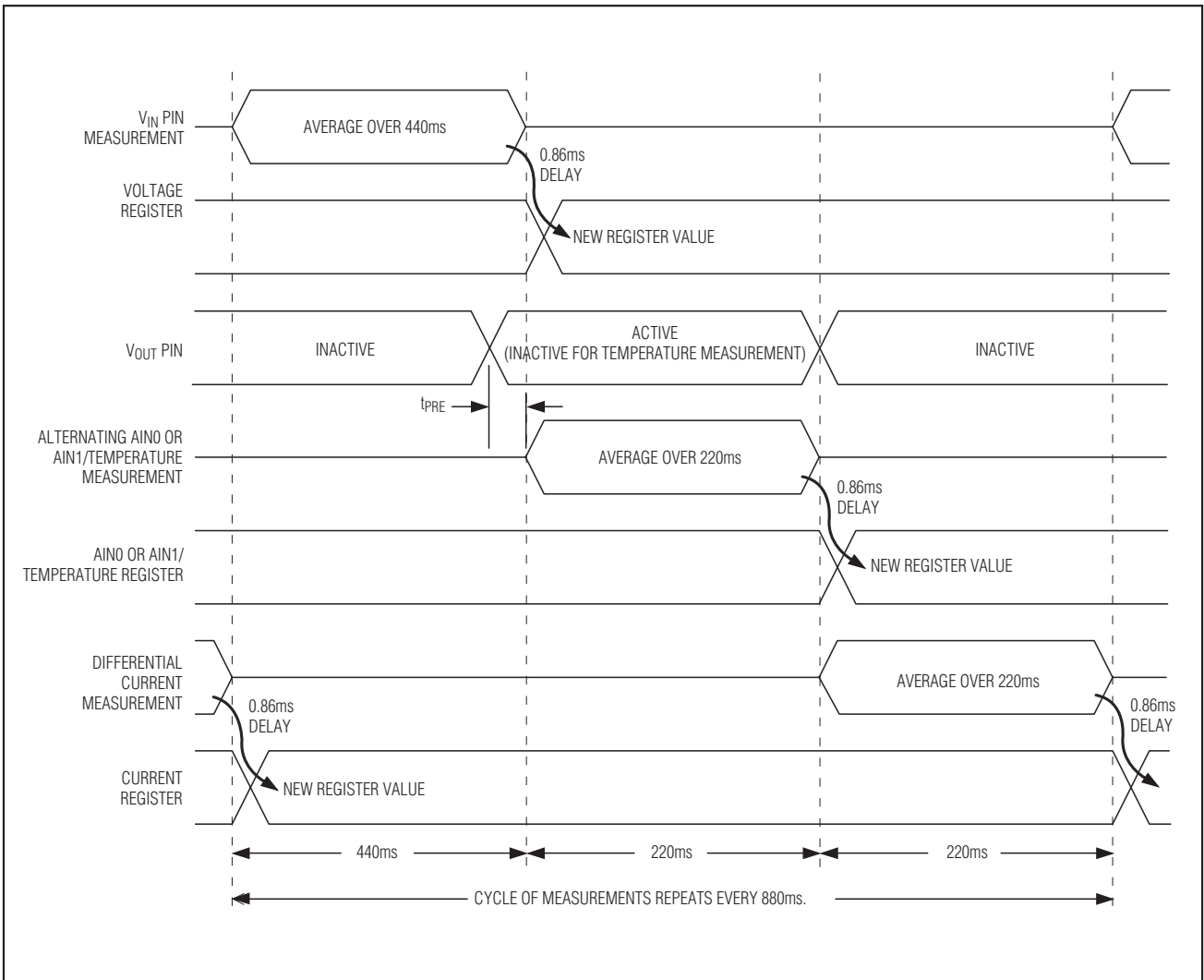
Figure 4. Measurement Sequence
