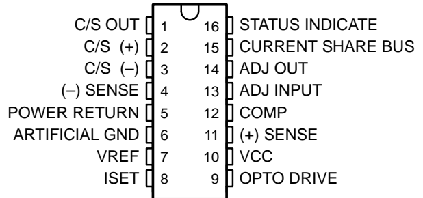
DIL-16 J or N PACKAGE (TOP VIEW)
