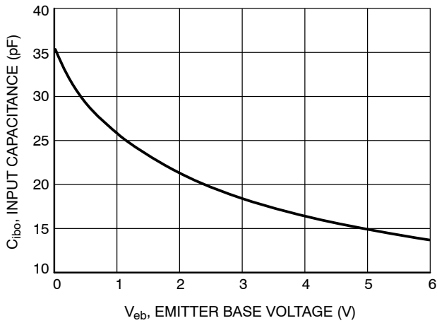
Figure 9. Input Capacitance vs. Emitter Base Voltage
