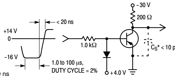
Figure 2. Turn–Off Time
