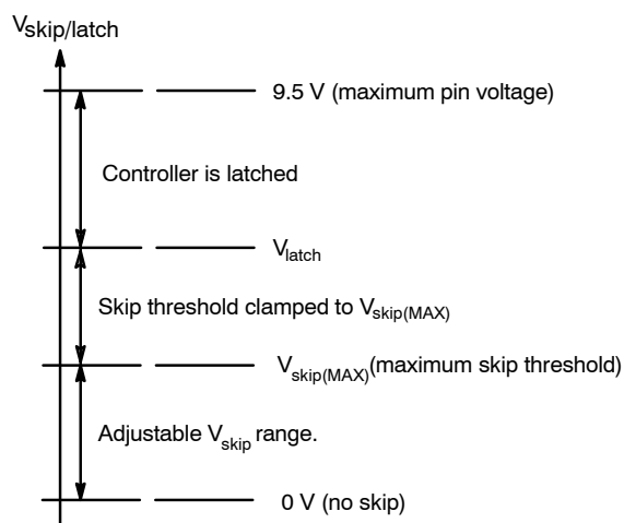
Figure 39. NCP1219 VSkip/latch Pin Operating Regions
