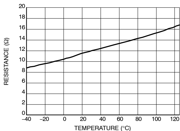
Figure 7. ROH
