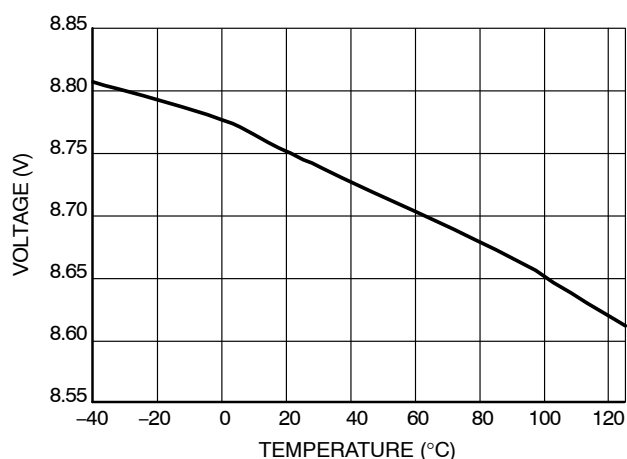
Figure 5. VBOOTon
