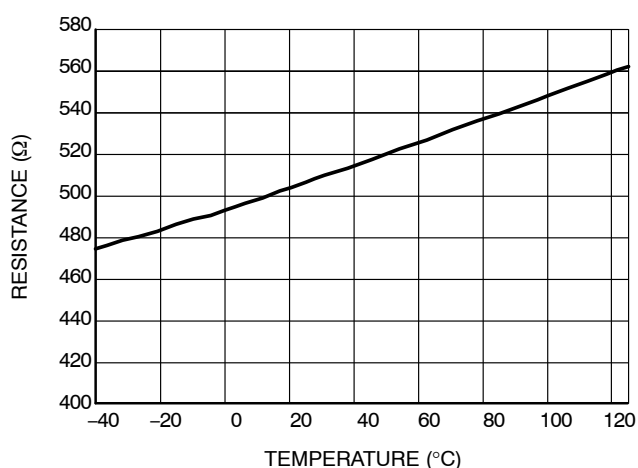
Figure 13. R T_discharge
