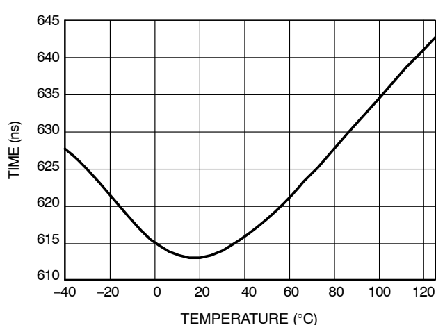
Figure 14. T dead
