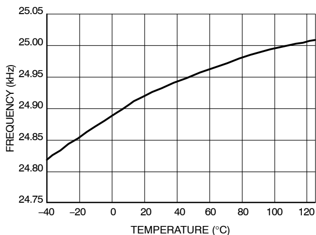
Figure 10. F SWmin
