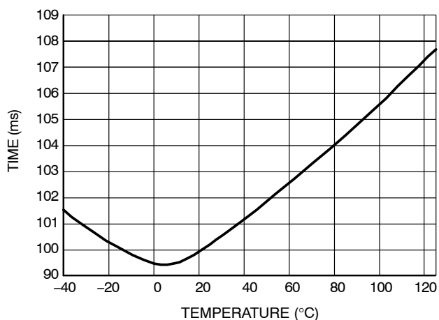
Figure 15. PFC delay
