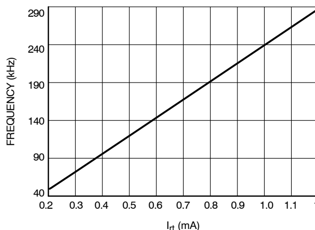
Figure 20. I rt and Appropriate Frequency
