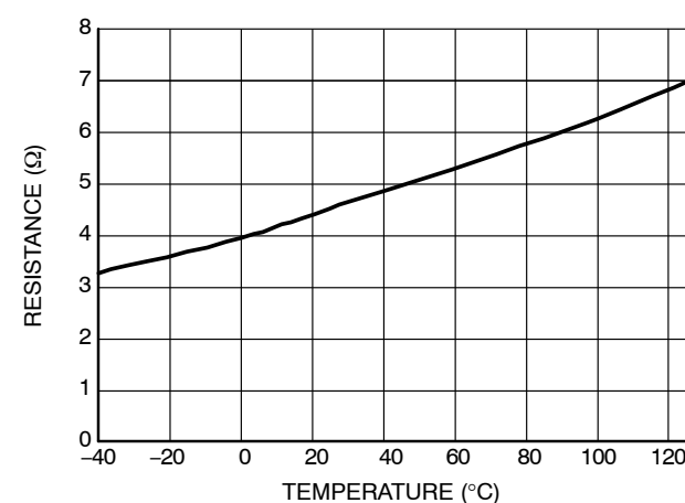
Figure 8. ROL
