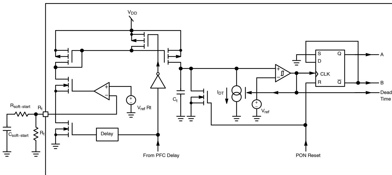
Figure 21. The Internal Current Controlled Oscillator Architecture
