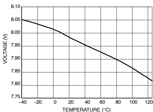
Figure 6. VBOOTmin
