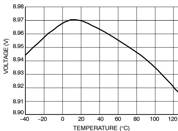
Figure 4. VCCmin
