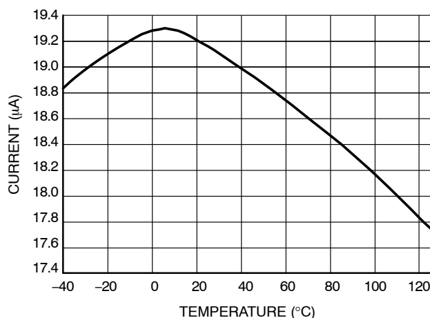
Figure 18. I BO
