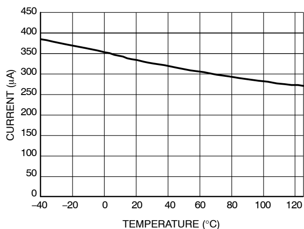
Figure 12. I CC4
