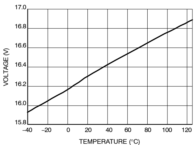
Figure 19. V CC_clamp
