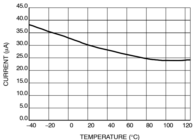
Figure 11. I CC_startup
