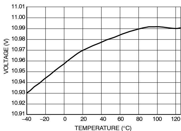
Figure 3. VCCon
