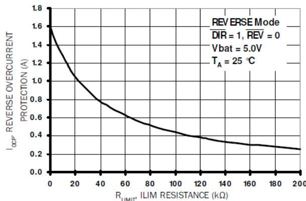
Figure 5. Reverse Mode Overcurrent Protection vs. ILIM Resistance, R_{\text{LIMIT}}
