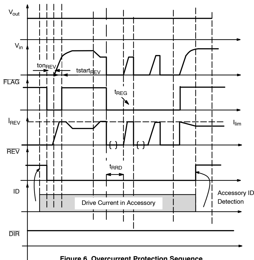
Figure 6. Overcurrent Protection Sequence
