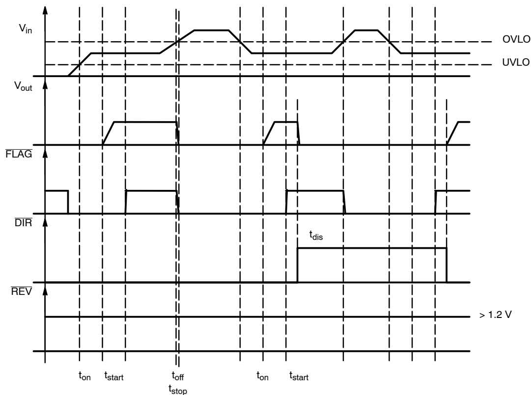
Figure 3. \overline{\text{FLAG}} Pin in AC/DC Charging Mode
