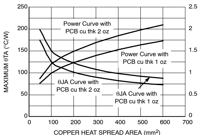
Figure 7. Copper heat Spread Area
