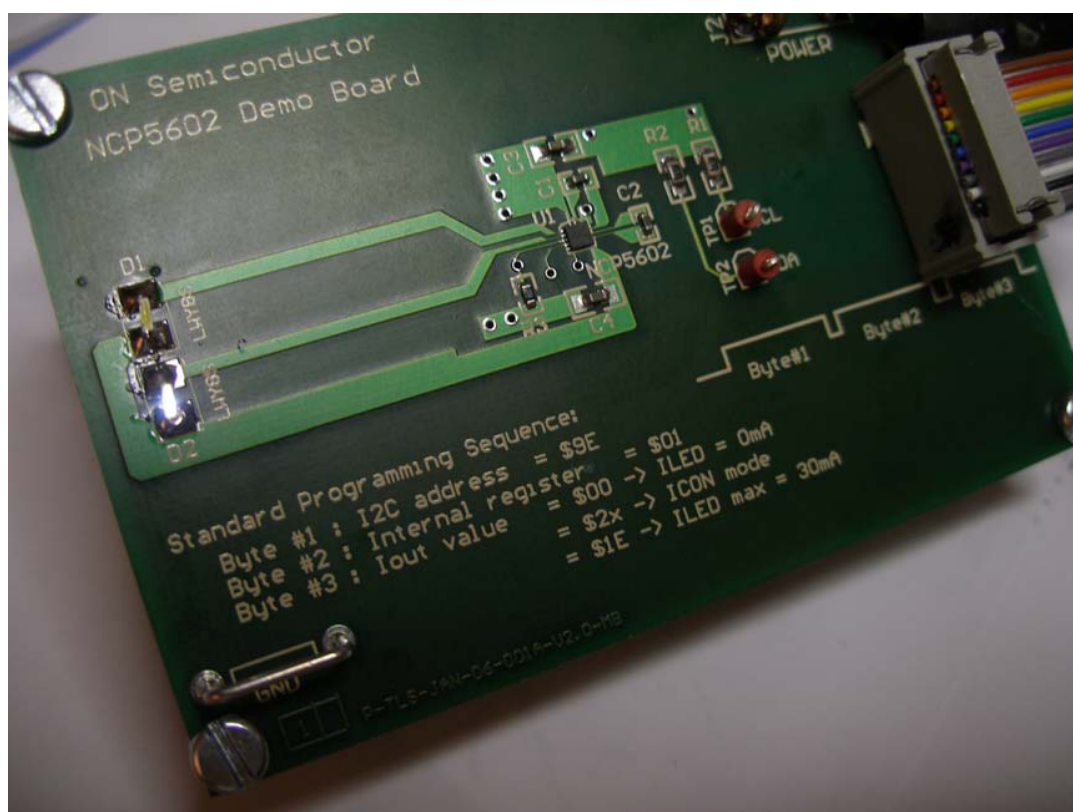
Figure 15. NCP5602 Demo Board
