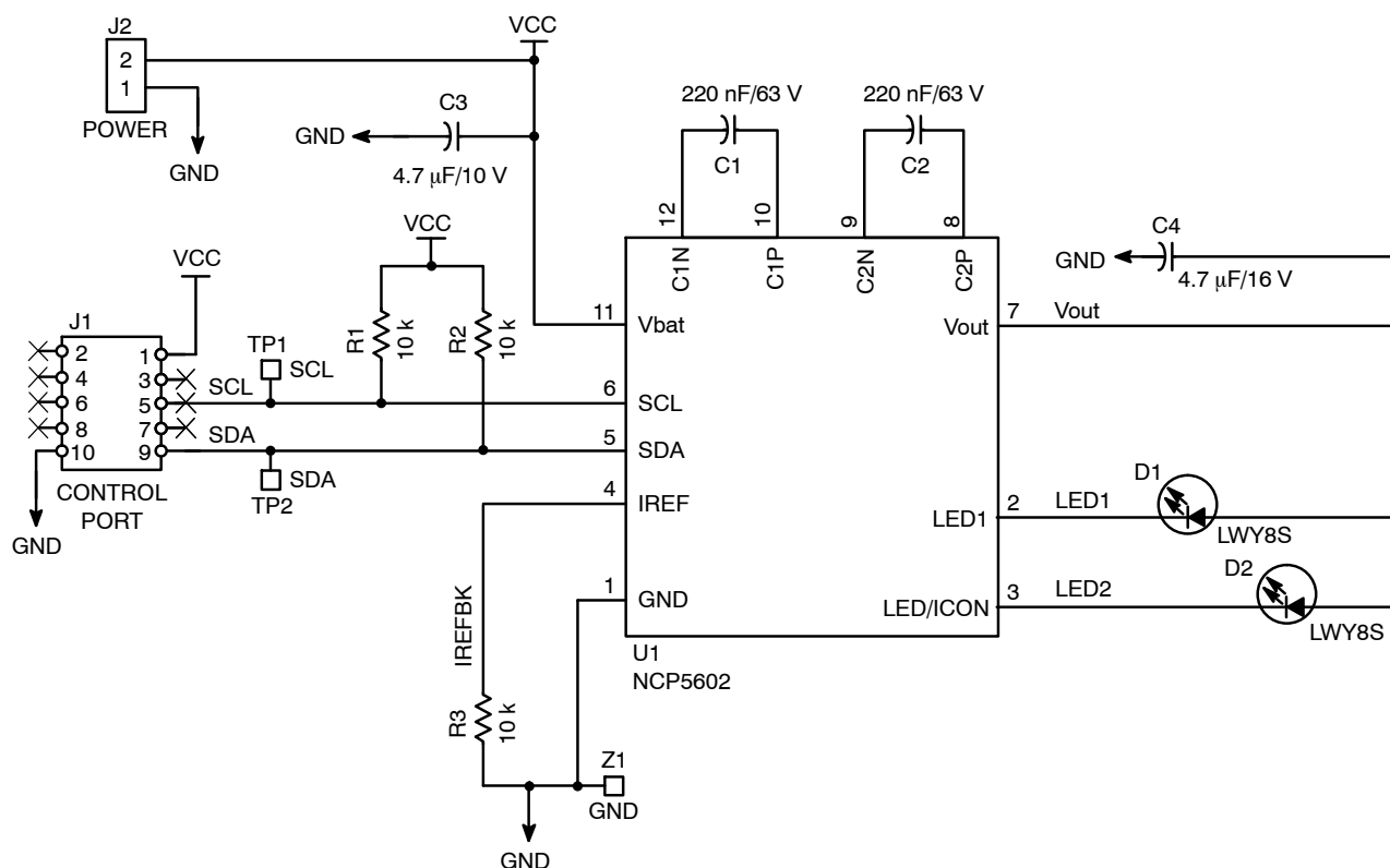
Figure 12. Demo Board Schematic Diagram
