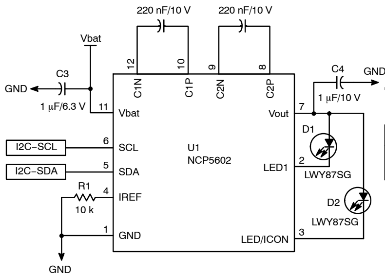
Figure 1. Typical Multiple White LED Driver
