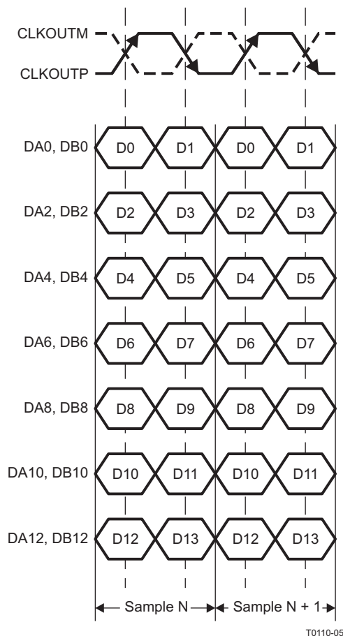
Figure 114. DDR LVDS Interface
