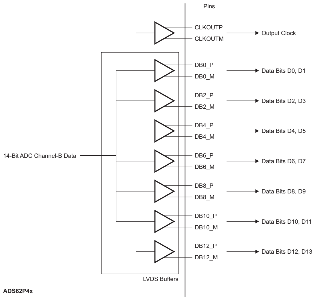
Figure 113. LVDS Outputs
