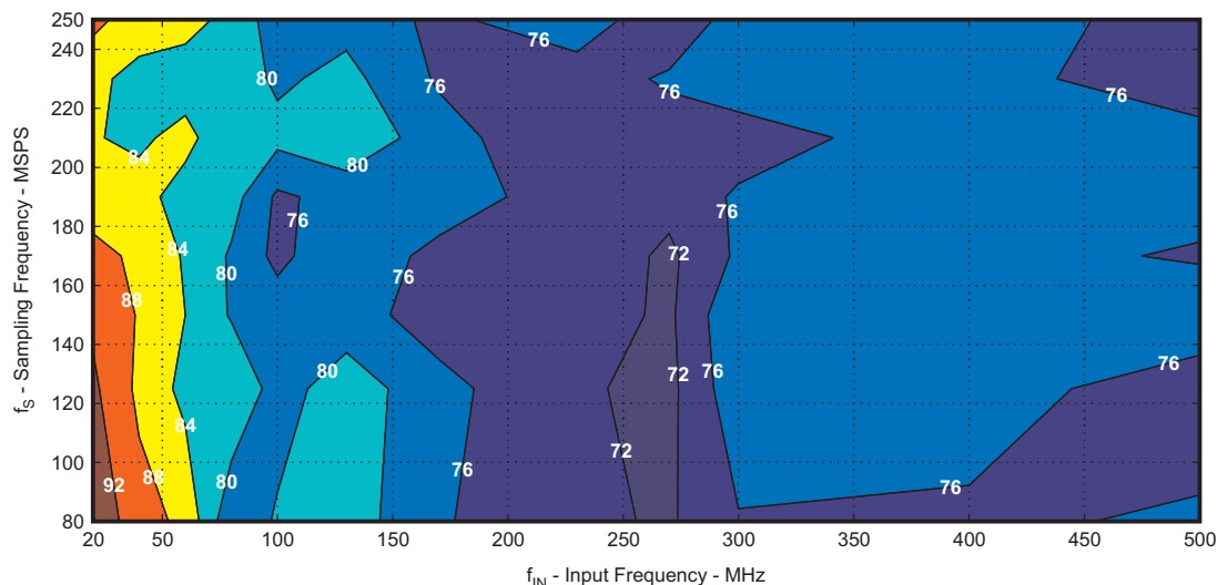
SFDR CONTOUR, 0 dB GAIN, UP TO 500 MHz
