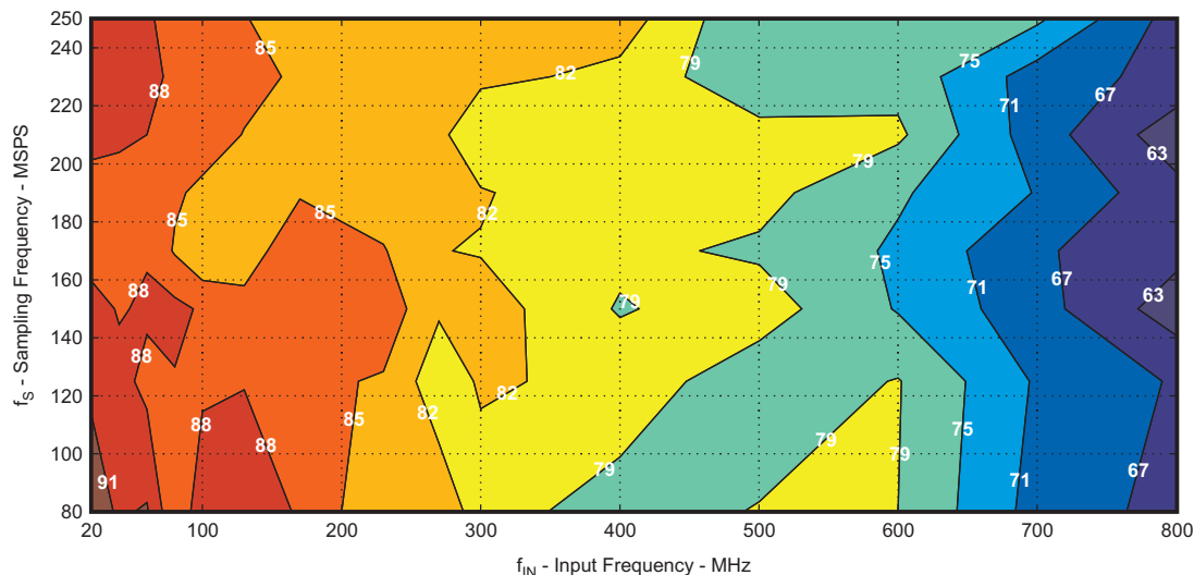
SFDR CONTOUR, 6 dB GAIN, UP TO 800 MHz
