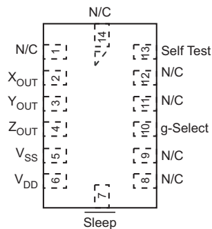
Figure 4. Pinout Description
