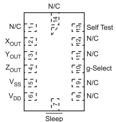
Figure 1. Pin Connections
