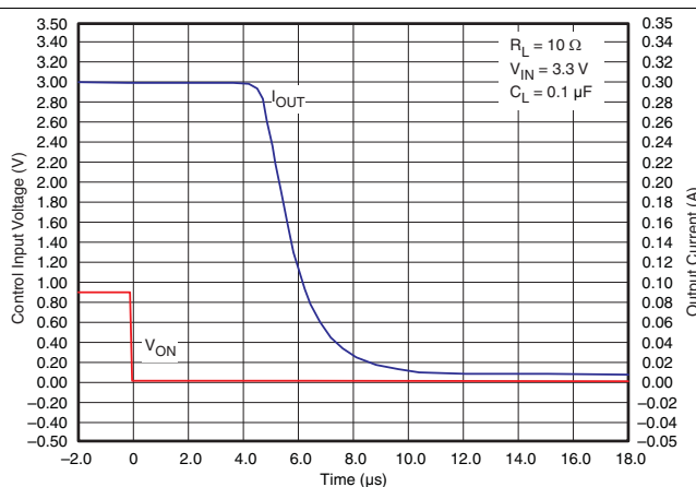
Figure 23. t_{OFF} Response
