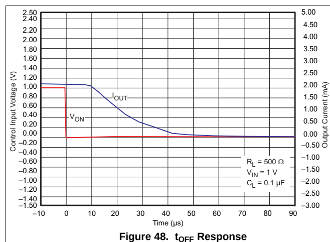
Figure 48. t_{OFF} Response
