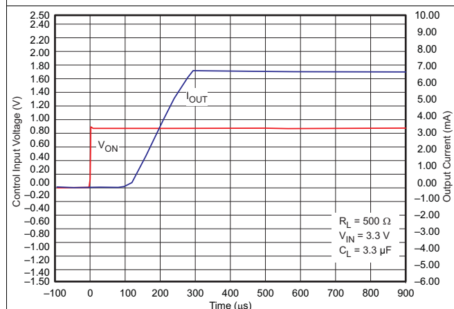
Figure 38. t_{ON} Response
