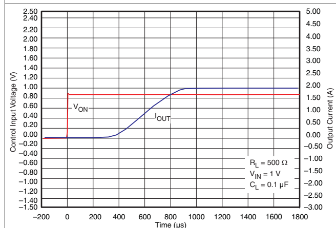
Figure 40. t_{ON} Response
