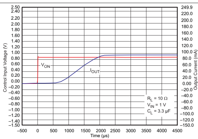
Figure 43. t_{ON} Response
