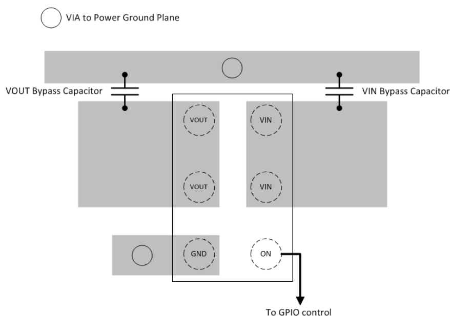
Figure 55. Layout Recommendation
