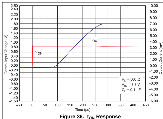
Figure 36. t_{ON} Response
