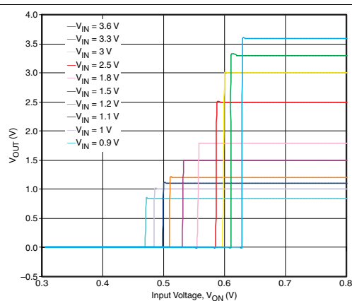
Figure 10. ON-Input Threshold
