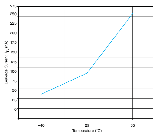
Figure 6. I_{IN} Leakage Current vs Temperature ( V_{IN} = 3.3 V)
