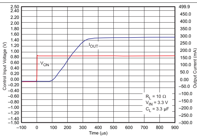
Figure 39. t_{ON} Response
