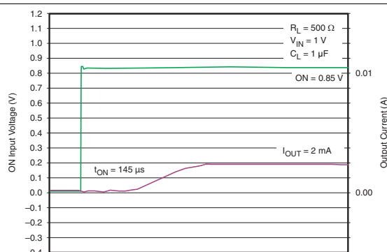
Figure 20. t_{ON} Response
