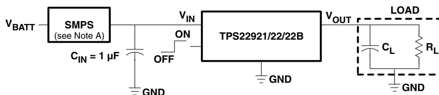
Figure 53. Typical Application
