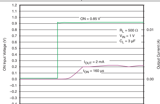
Figure 21. t_{ON} Response
