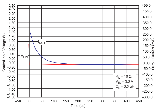
Figure 47. t_{OFF} Response
