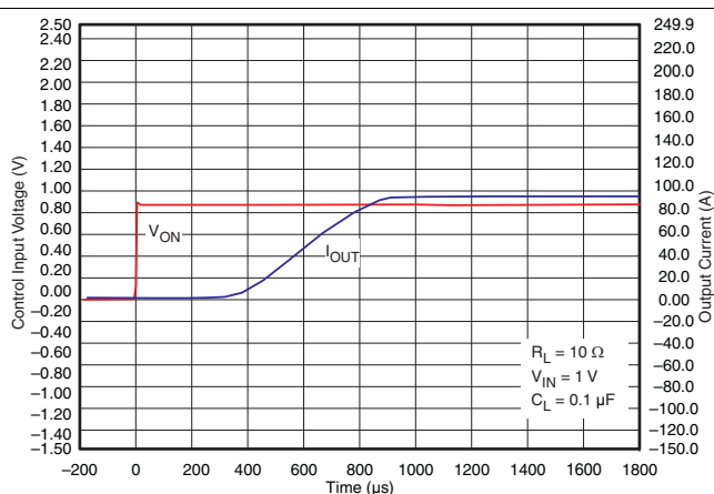
Figure 41. t_{ON} Response
