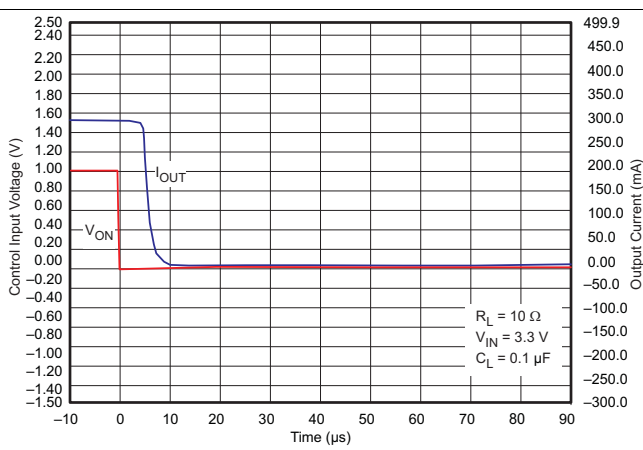
Figure 45. t_{OFF} Response
