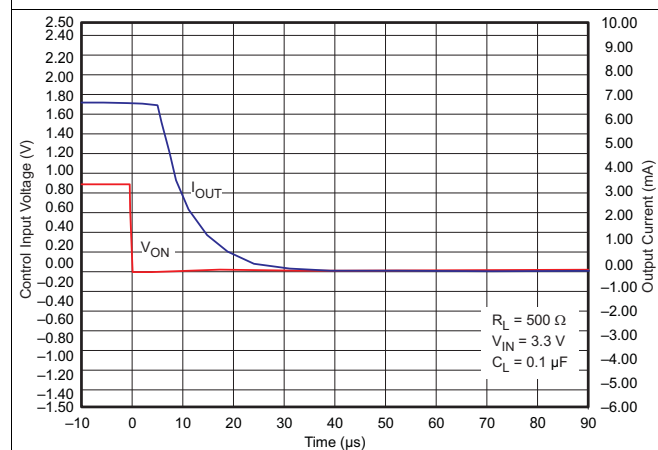
Figure 44. t_{OFF} Response
