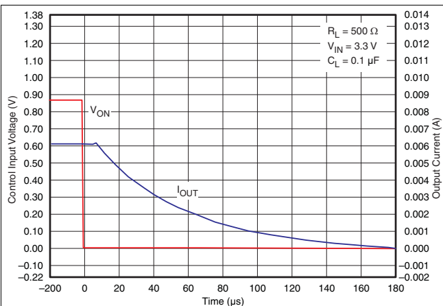
Figure 22. t_{OFF} Response
