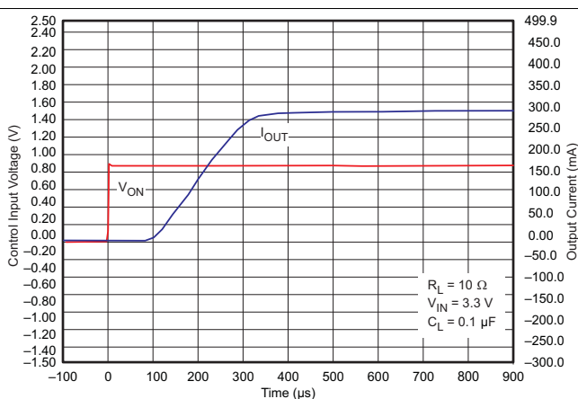
Figure 37. t_{ON} Response
