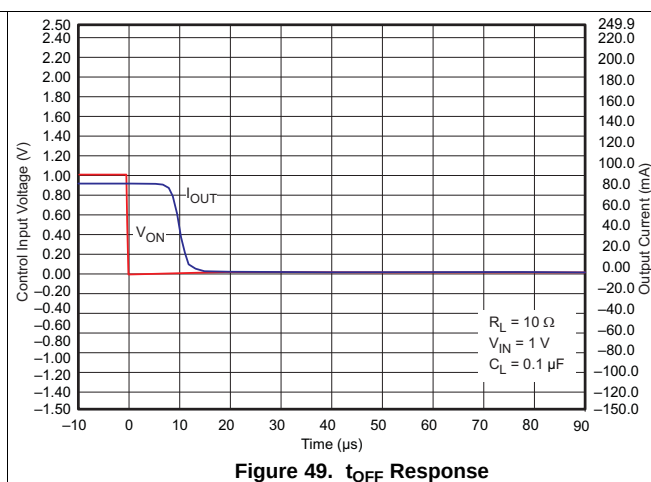
Figure 49. t_{OFF} Response
