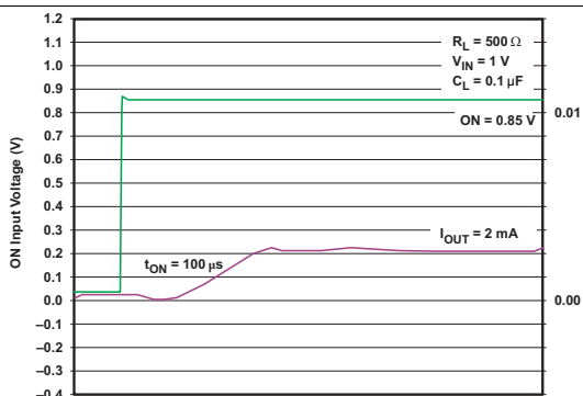
Figure 19. t_{ON} Response
