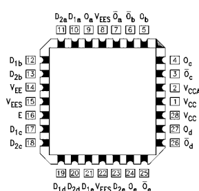
28-Pin PLCC
