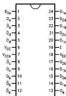
24-Pin DIP/SOIC
