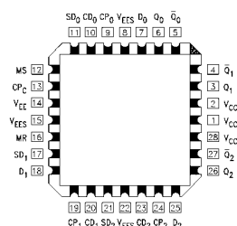
28-Pin PLCC
