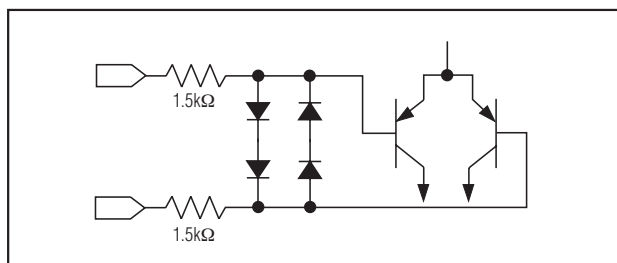
Figure 2. Input Protection Circuit
