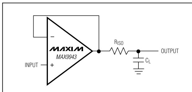
Figure 1. Capacitive Load Driving Circuit
