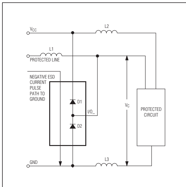
Figure 6. Layout Considerations
