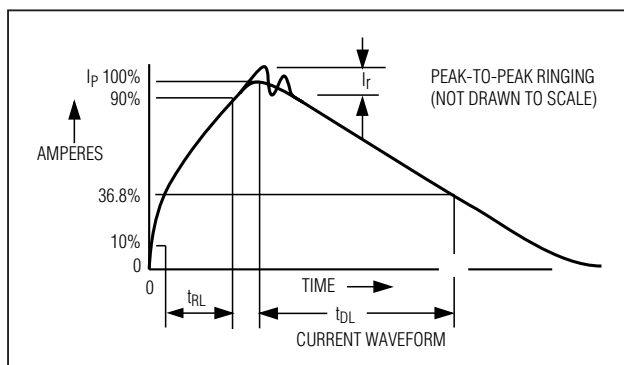
Figure 4. Human Body Model Current Waveform
