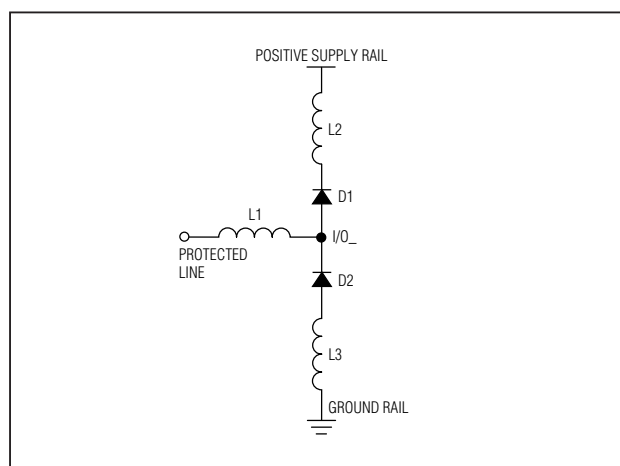
Figure 1. Parasitic Series Inductance
