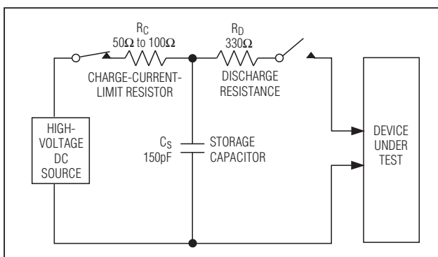
Figure 5. IEC 61000-4-2 ESD Test Model
