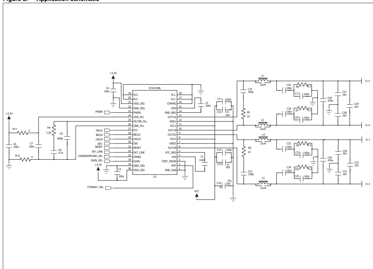
Figure 8. Application schematic
