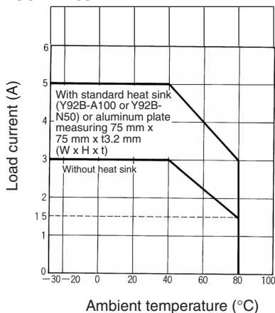
G3NA-240B
