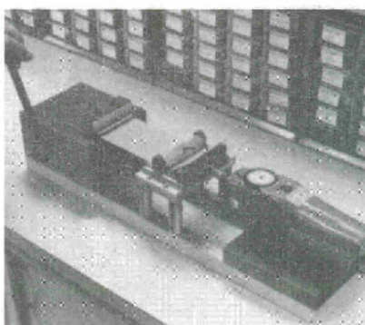
Test to determine the force for cover pull-off from base of connector
