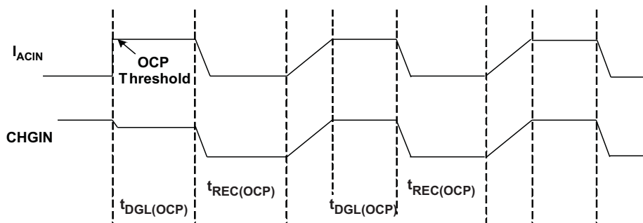
Figure 14. Charge Current OCP Timing Diagram
