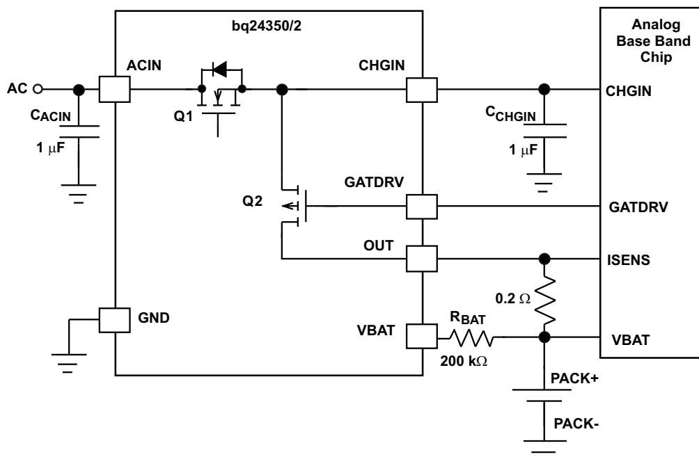
Figure 1. Host Controlled One-Cell Charger Application Circuit
