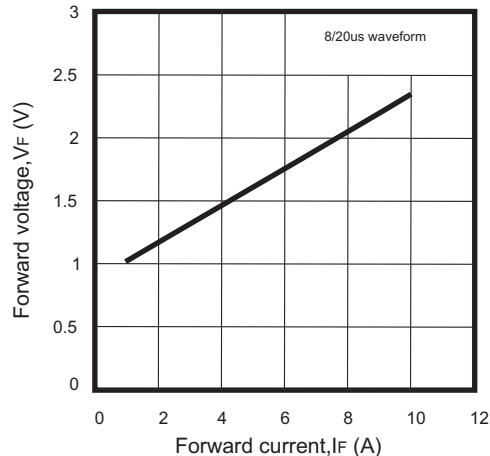
Fig. 4 - Forward volatage vs. forward current
