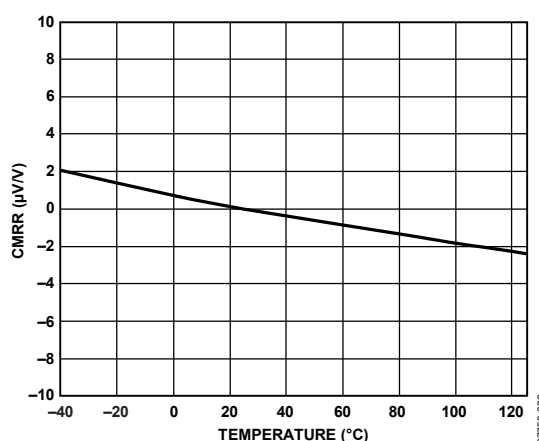
Figure 32. CMRR vs. Temperature, G = 5
