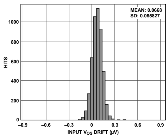
Figure 6. Typical Distribution of Input Offset Voltage Drift, G = 100
