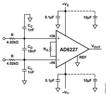
Figure 63. RFI Suppression
