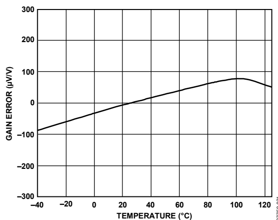
Figure 31. Gain Error vs. Temperature, G = 5
