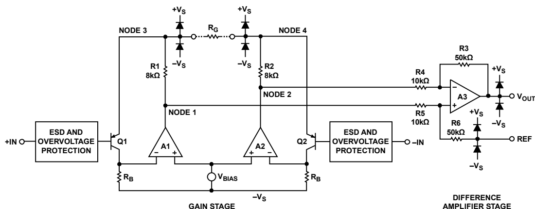
Figure 58. Simplified Schematic
