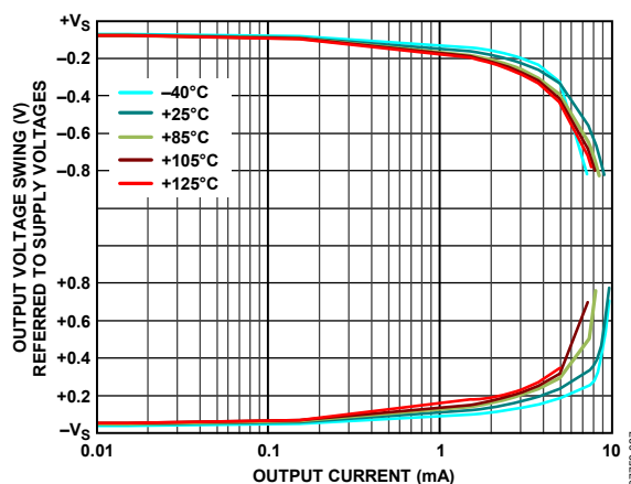
Figure 37. Output Voltage Swing vs. Output Current
