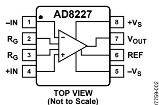
Figure 2. Pin Configuration
