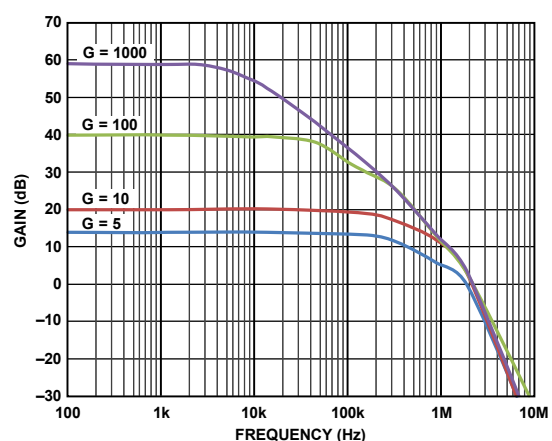
Figure 26. Gain vs. Frequency, V_s = 2.7\text{ V}
