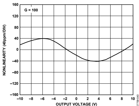
Figure 40. Gain Nonlinearity, G = 100 , R_L \geq 2 \text{ k}\Omega
