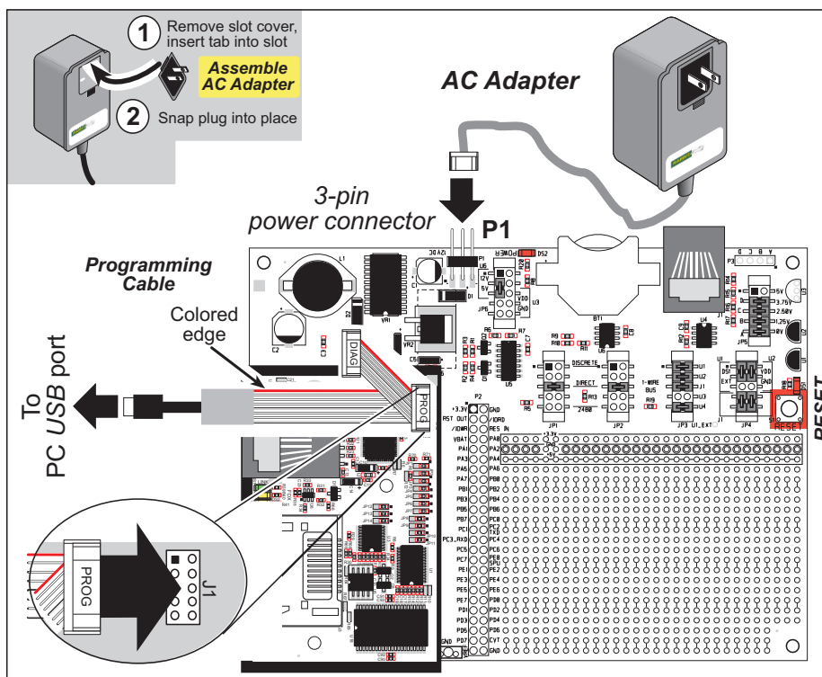
Figure 3. Connect Programming Cable and Power Supply
