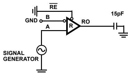
FIGURE 6A. TEST CIRCUIT
