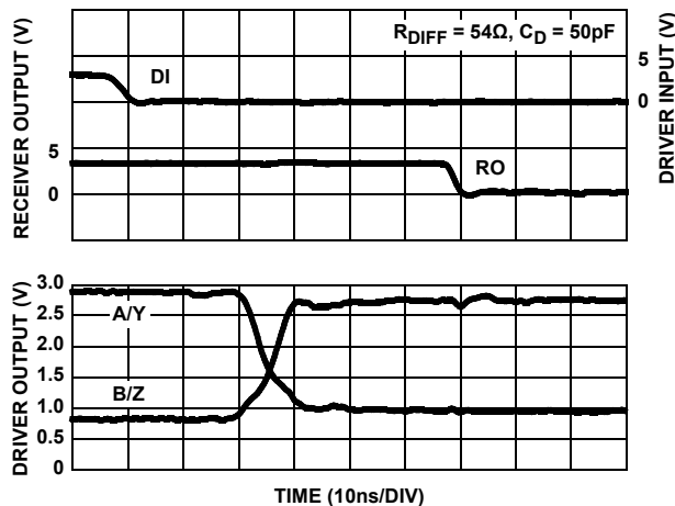
FIGURE 15. DRIVER AND RECEIVER WAVEFORMS, HIGH-TO-LOW
