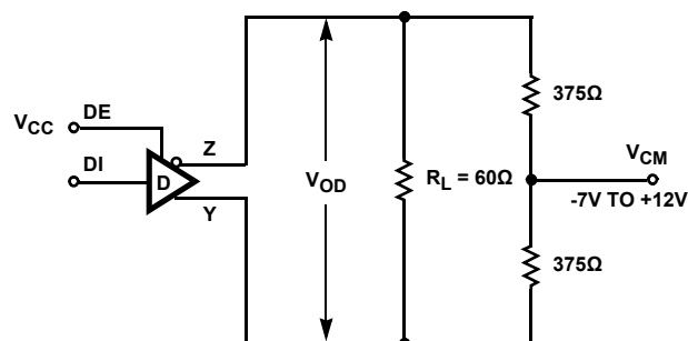
FIGURE 2B. V_{OD} WITH COMMON MODE LOAD
