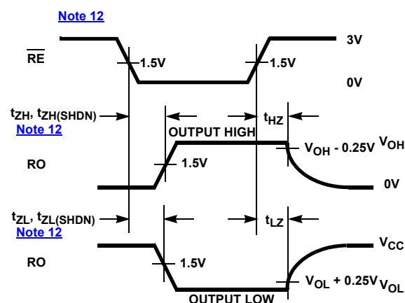
FIGURE 7B. MEASUREMENT POINTS
