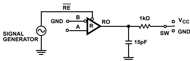
FIGURE 6. RECEIVER PROPAGATION DELAY
