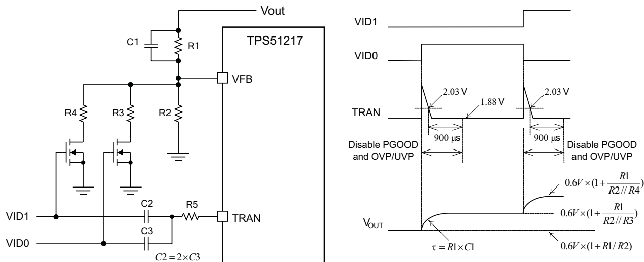
Figure 22. Dynamic Voltage Step Application
