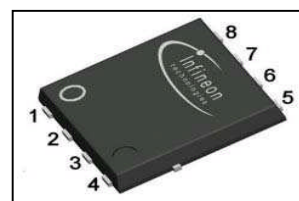
PG-TDSO8
