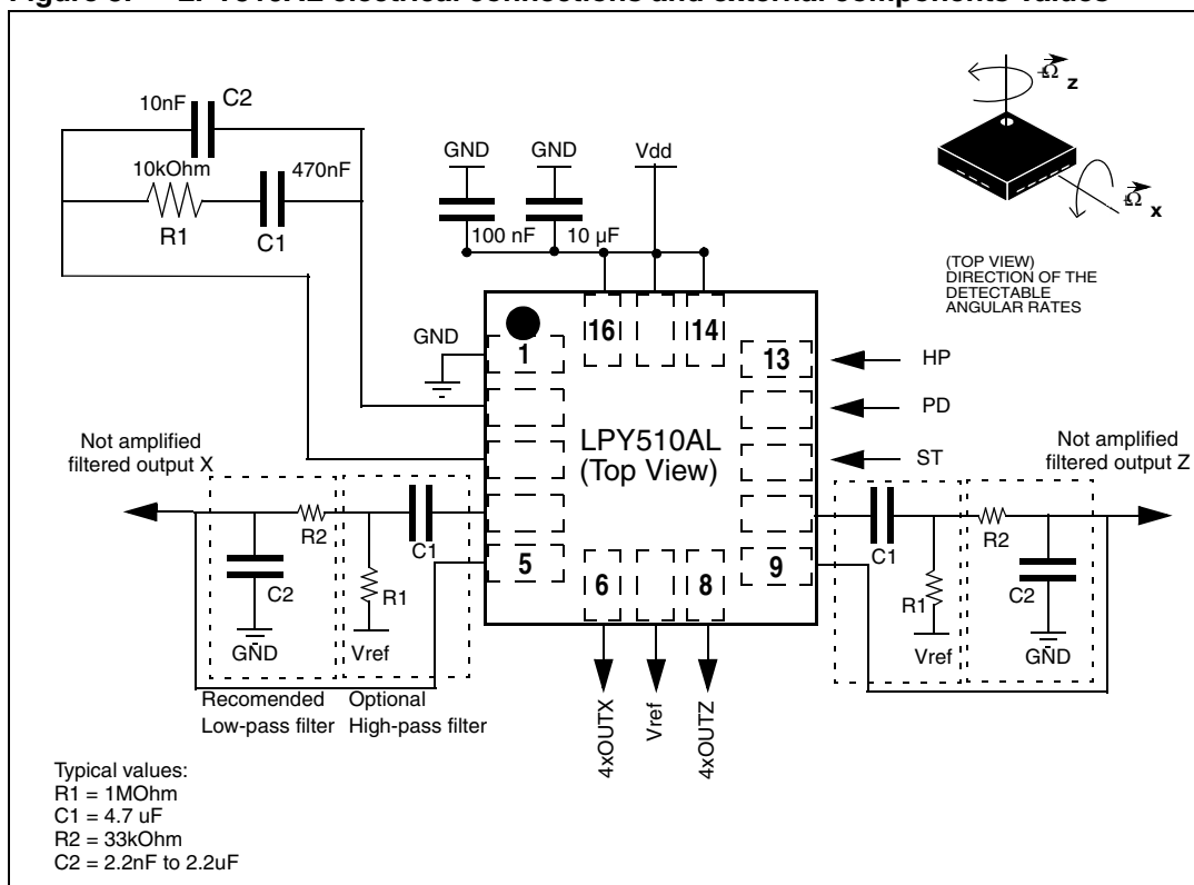
Figure 3. LPY510AL electrical connections and external components values
