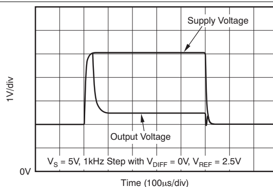
Figure 20. Noninverting Differential Input Overload
