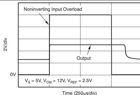
Figure 20. Noninverting Differential Input Overload
