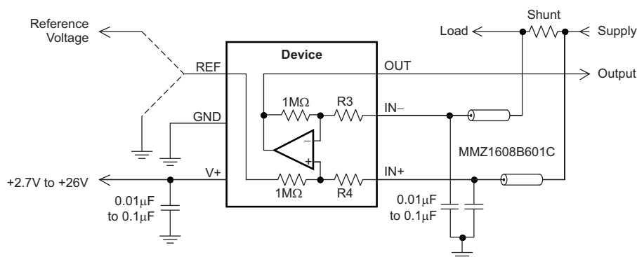
Figure 29. Transient Protection
