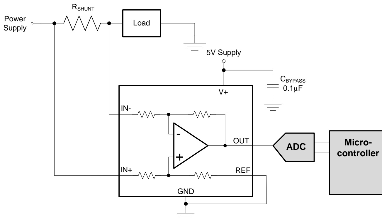
Figure 23. Typical Application
