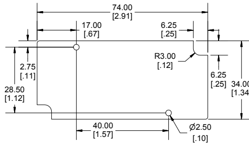
MAXIMUM P.C. BOARD SIZE
