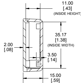
END VIEW SECTION B-B
