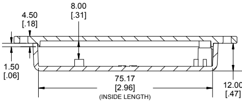
SIDE VIEW SECTION A-A
