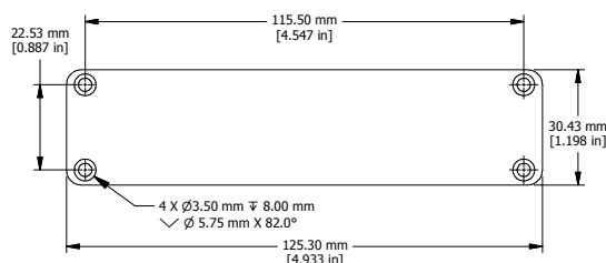
END PLATE
