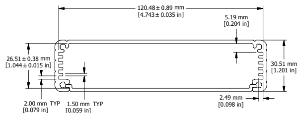
EXTRUSION
