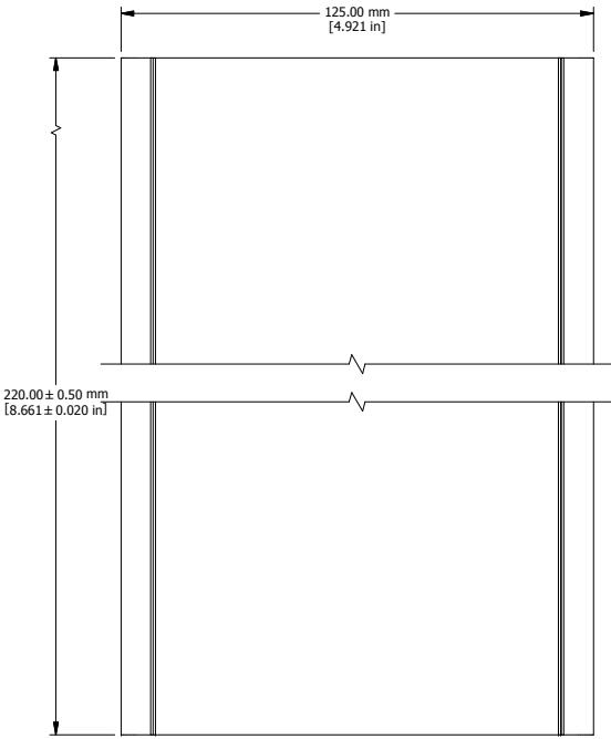
EXTRUSION DESIGNED FOR 120MM WIDE PC BOARD
