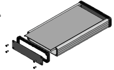
EXPLODED ASSEMBLY VIEW
