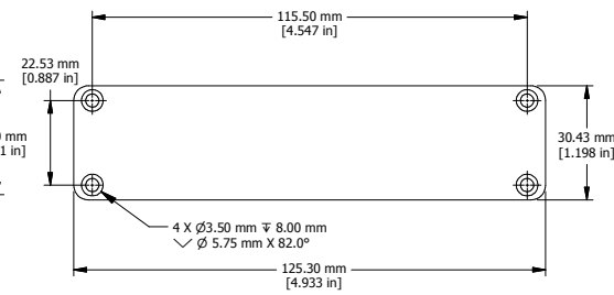
END PLATE
