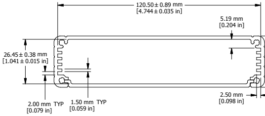
EXTRUSION
