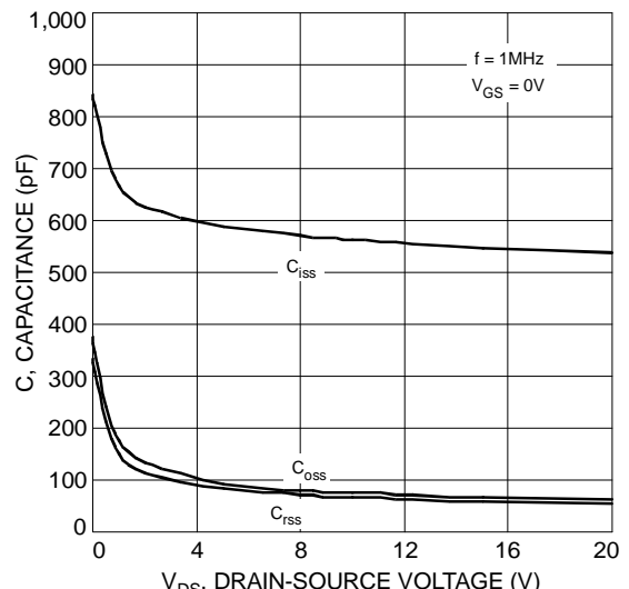
Fig. 6 Typical Capacitance
