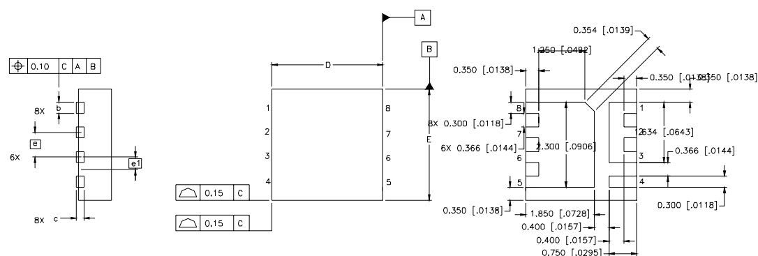
SIDE VIEW
