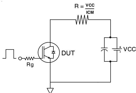
Fig.C.T.2 - RBSOA Circuit
