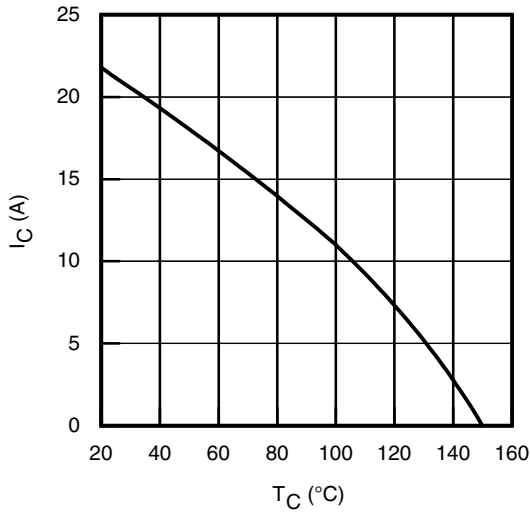
Fig 7. Maximum Collector Current vs. Case Temperature
