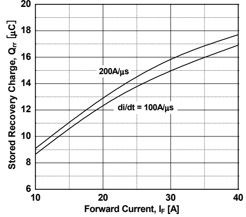
Figure 20. Stored Charge
