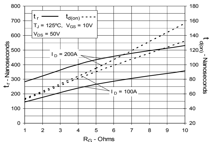
Fig. 14. Resistive Turn-on Switching Times vs. Gate Resistance
