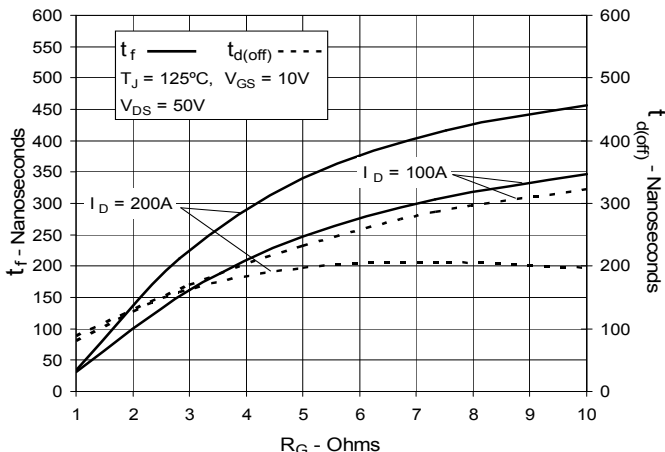
Fig. 17. Resistive Turn-off Switching Times vs. Gate Resistance
