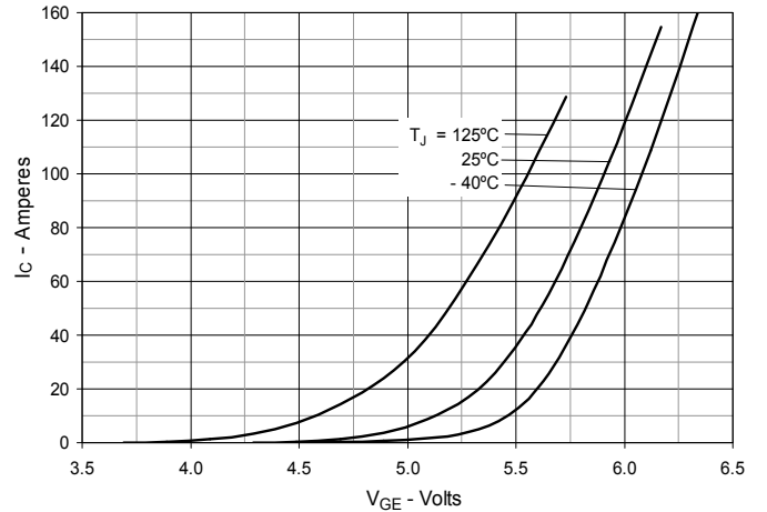
Fig. 6. Input Admittance
