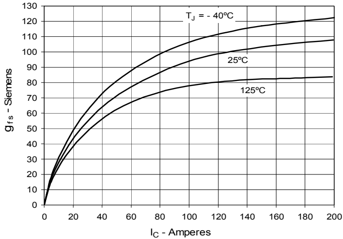
Fig. 7. Transconductance
