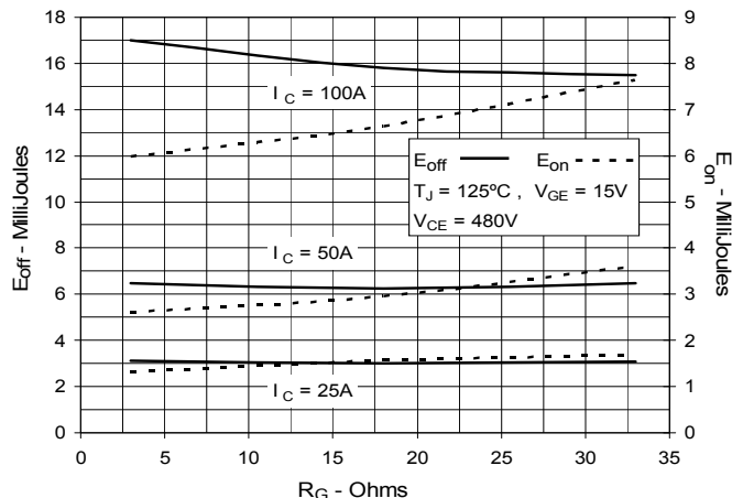
Fig. 12. Inductive Switching Energy Loss vs. Gate Resistance
