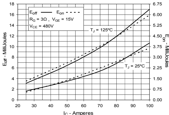
Fig. 13. Inductive Switching Energy Loss vs. Collector Current
