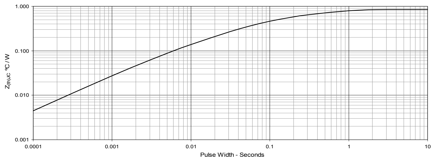
Fig. 27. Maximum Transient Thermal Impedance (for diode)
