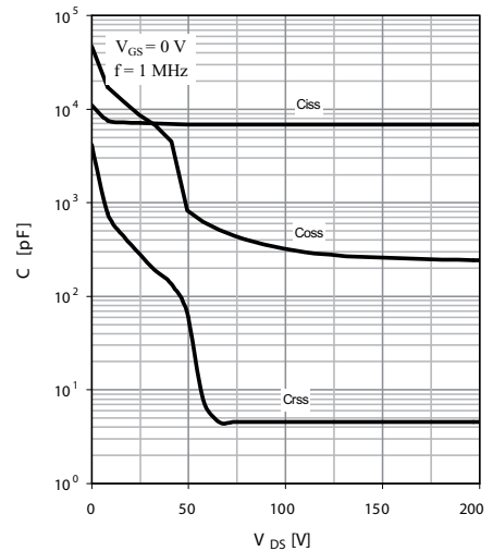
Fig. 9 Typ. capacitances
