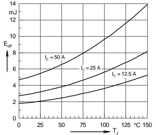
Fig. 11 Typ. turn-off energy per pulse
