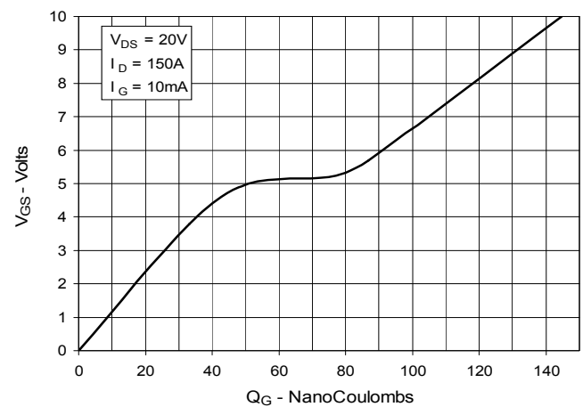
Fig. 10. Gate Charge
