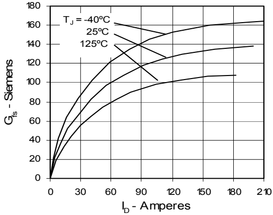
Fig. 7. Transconductance
