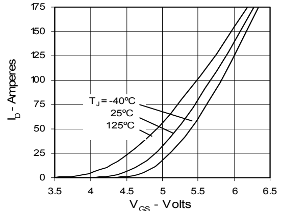
Fig. 6. Input Admittance
