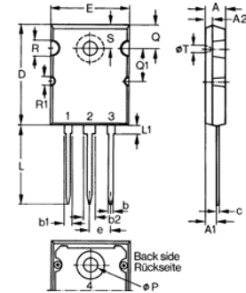
TO-264 AA Outline
