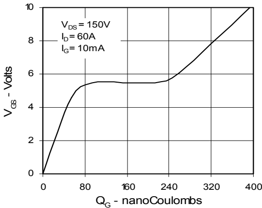
Fig. 9. Gate Charge
