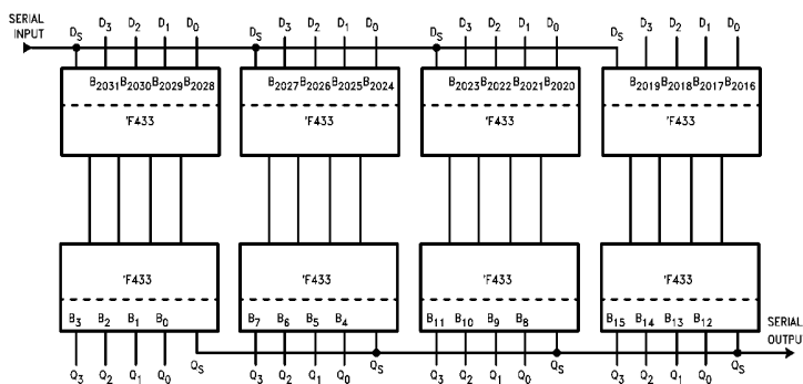
FIGURE 9. Final Position of a 2032-Bit Serial Input
