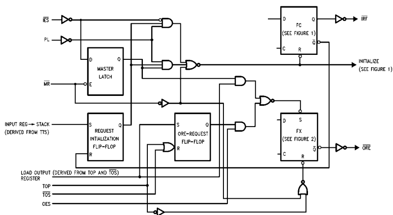
FIGURE 10. Conceptual Diagram, Interlocking Circuitry
