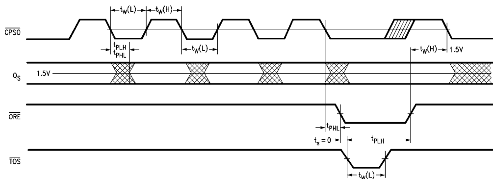
FIGURE 13. Serial Output, Unexpanded or Master Operation
