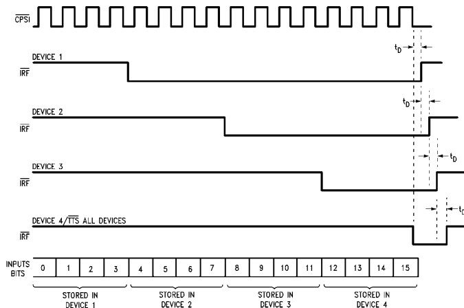
FIGURE 7. Serial Data Entry for Array of Figure 4
